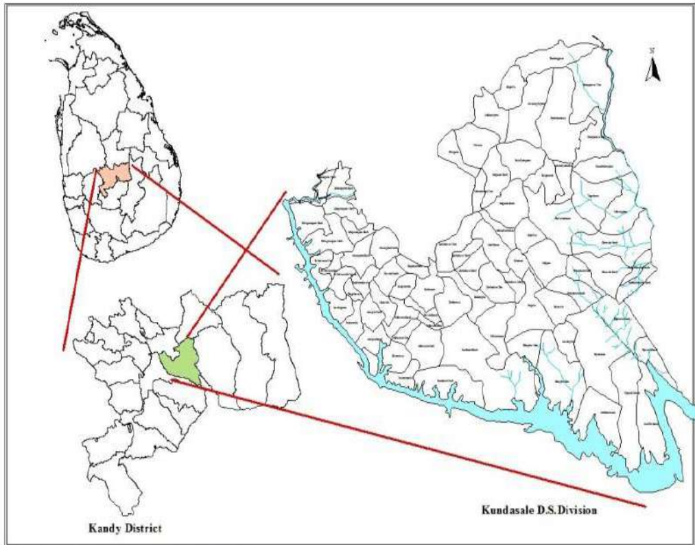
Fig 1. Location Map- Kandasale D.S.Division
